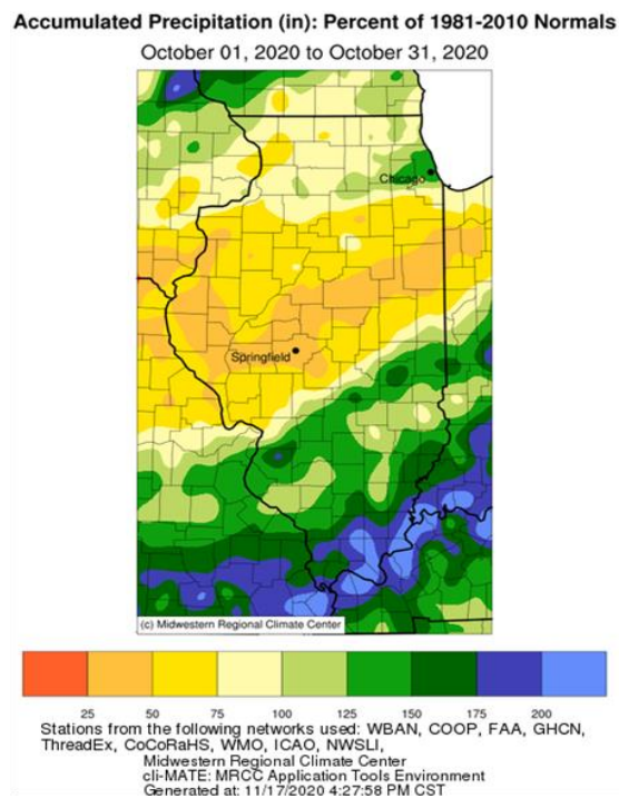
Figure 38: Accumulate precipitation (in.) for October, 2020
