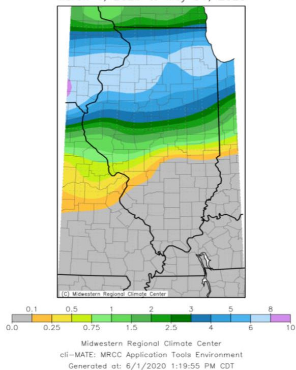
Accumulated Snowfall (in) March 1, 2020 to May 31, 2020
