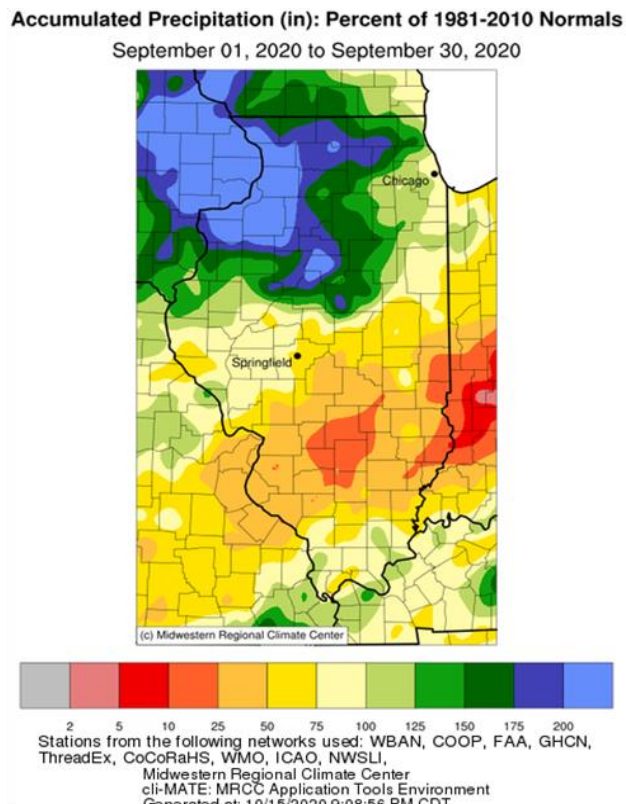
Figure 37: Accumulated precipitation (in.) for September, 2020
